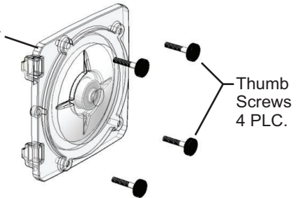
Pump Head Cover
