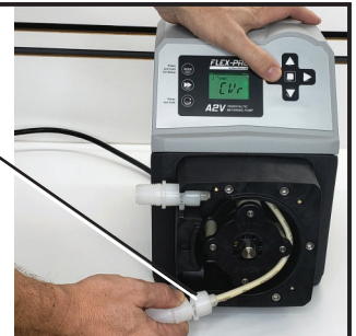
Suction side tube adapter
