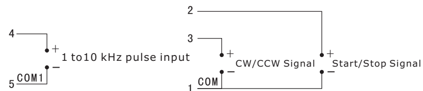
1 to 10 kHz Pulse Signal Input Connection Diagram
