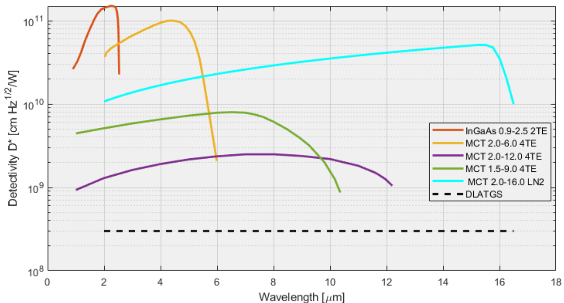
Specific detectivity ( D^* ) of ARcoptix detectors
