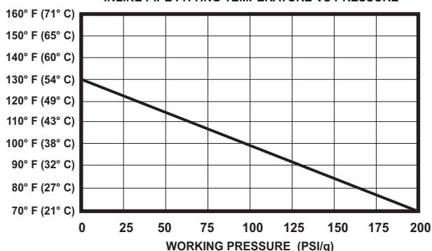
INLINE PIPE FITTING TEMPERATURE VS PRESSURE
