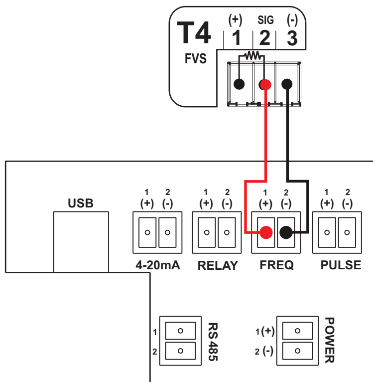
S6A Meter Board
